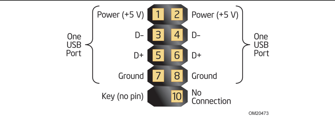
Figure 15. Connection Diagram for Front Panel USB 2.0 Headers
