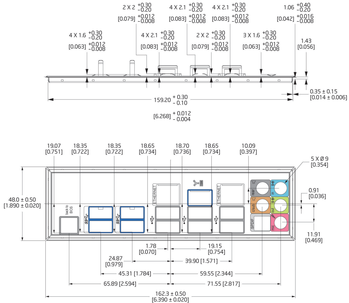
Figure 12. I/O Shield Reference Diagram
