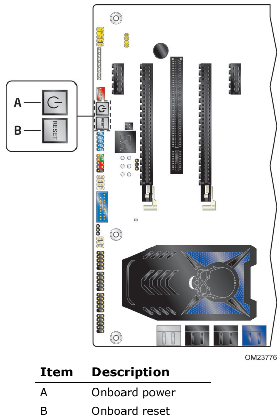
Figure 9. Location of the Onboard Power and Reset Buttons
