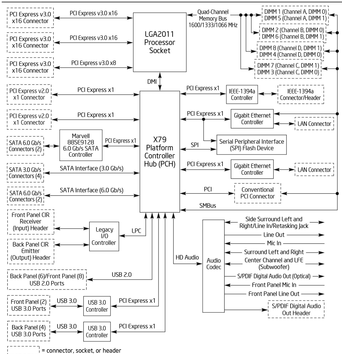
Figure 2. Block Diagram
