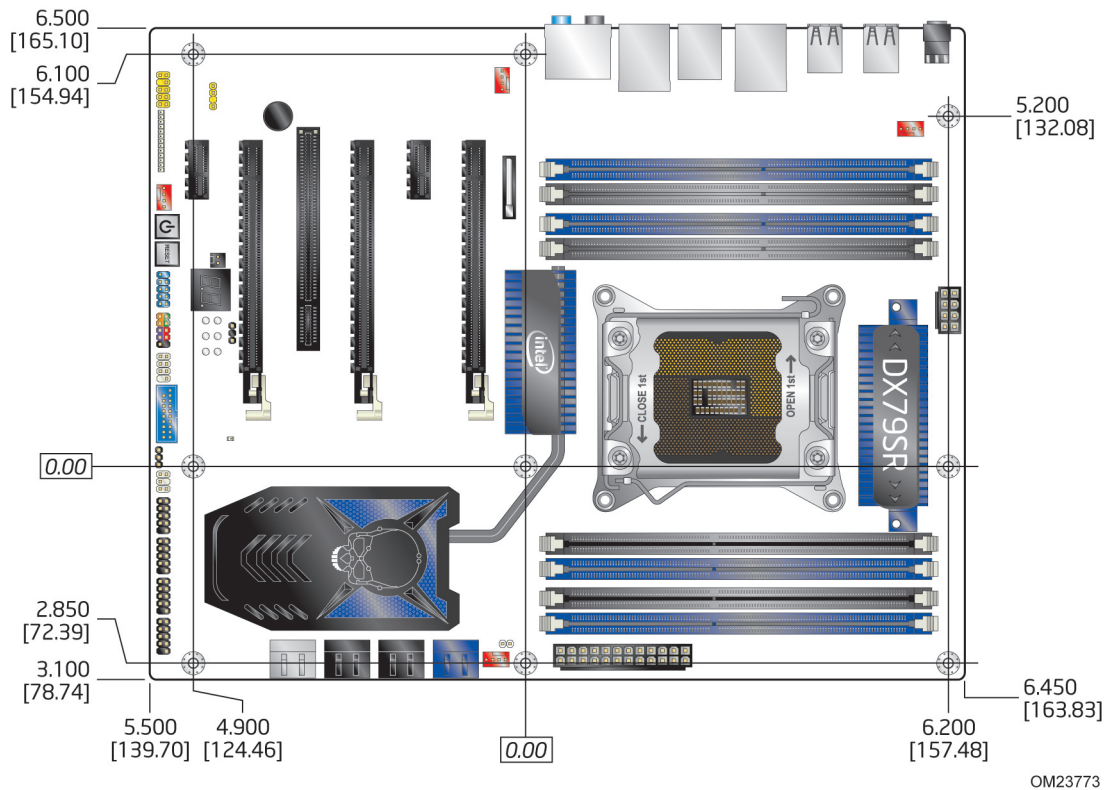
Figure 17. Board Dimensions
