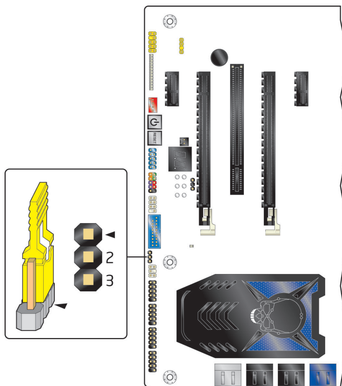
Figure 16. Location of the Jumper Block
