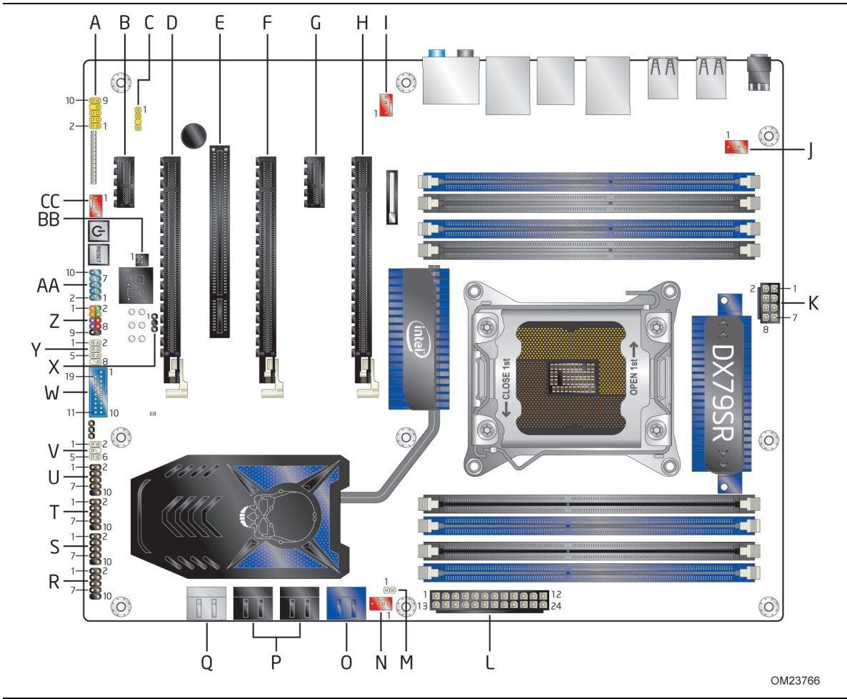
Figure 13. Component-side Connectors and Headers
