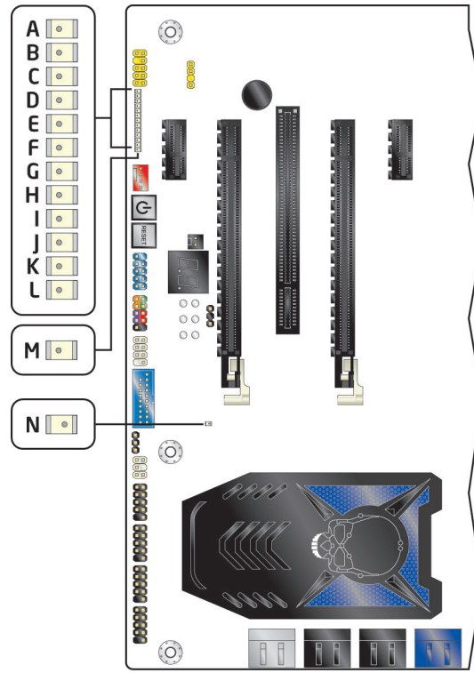
Figure 8. Location of Board Status LEDs
