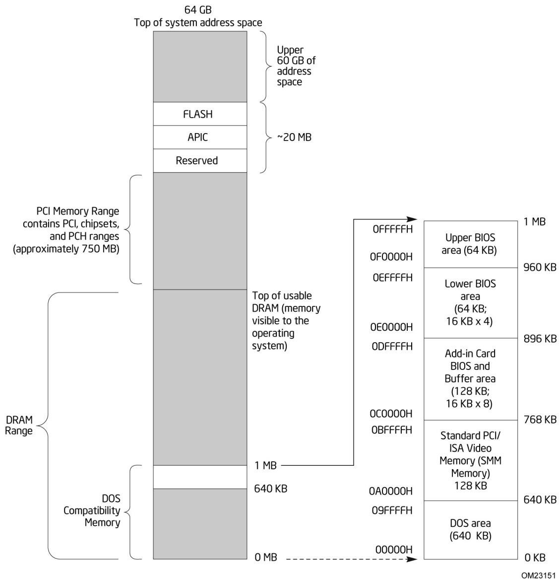
Figure 10. Detailed System Memory Address Map
