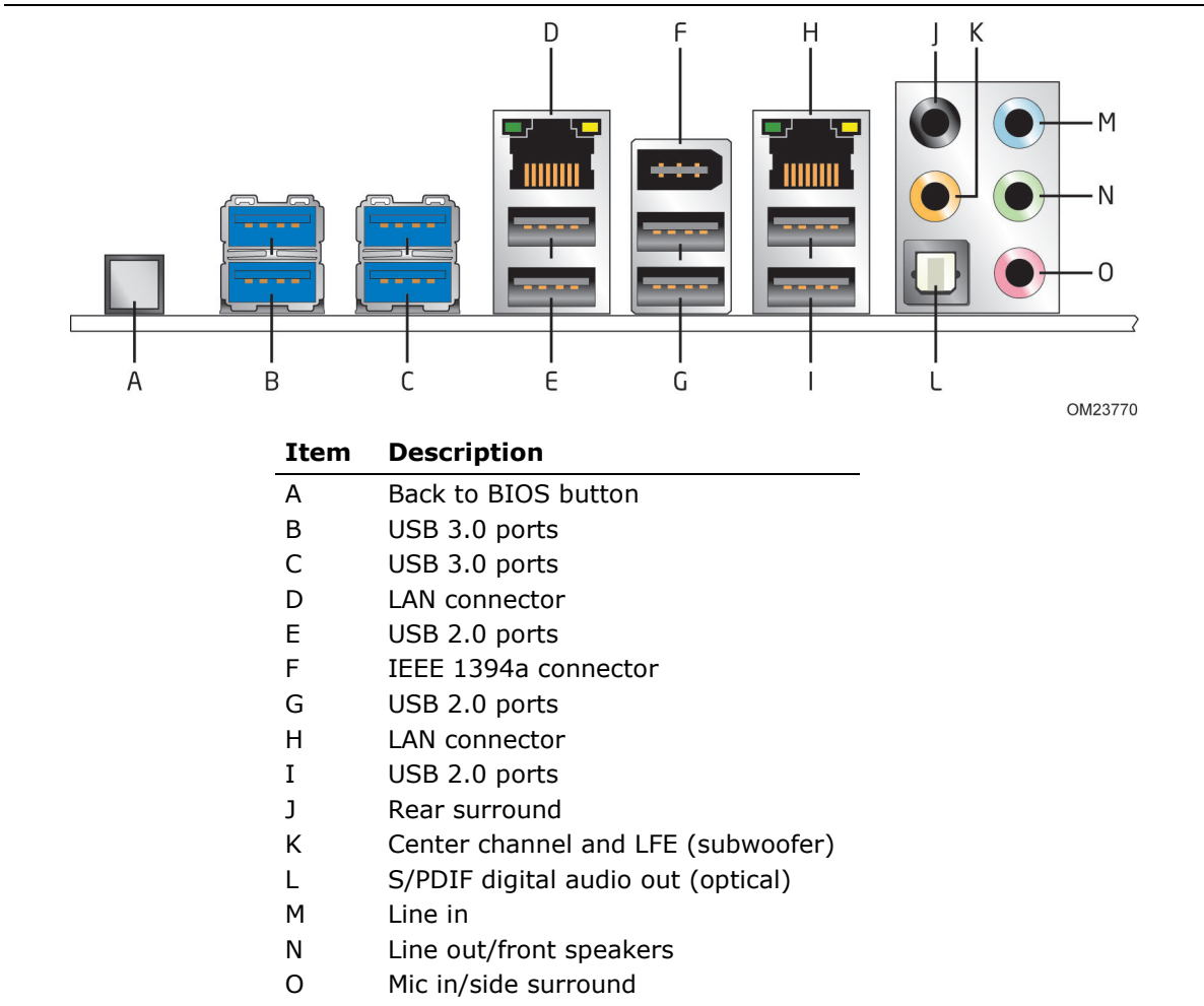
Figure 11. Back Panel Connectors
